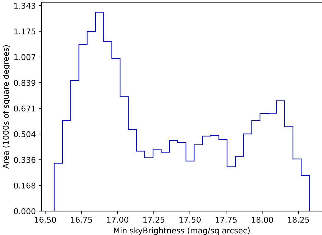
ddf_loaded_half_fl15_v3.4_10yrs WFD z band: Min skyBrightness
