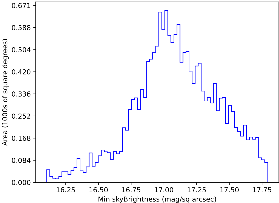
ddf_loaded_half_fl15_v3.4_10yrs WFD y band: Min skyBrightness
