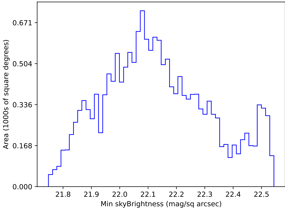
ddf_loaded_half_fl15_v3.4_10yrs WFD u band: Min skyBrightness
