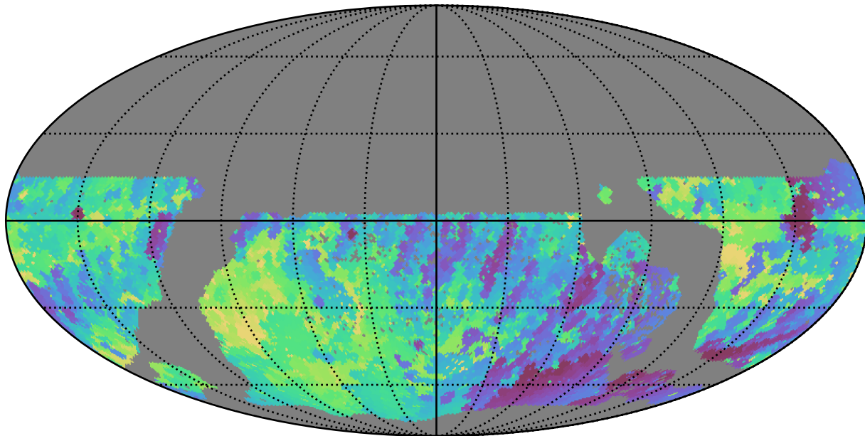
ddf_loaded_half_fl15_v3.4_10yrs WFD r band: Min skyBrightness
