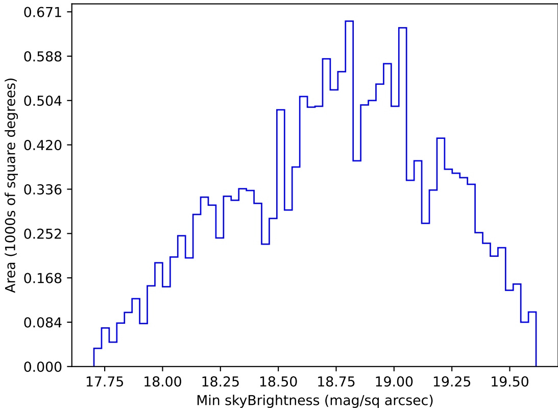
ddf_loaded_half_fl15_v3.4_10yrs WFD r band: Min skyBrightness
