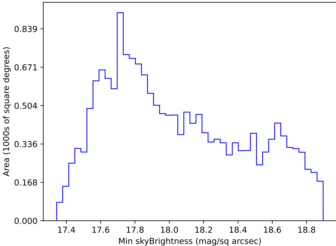
ddf_loaded_half_fl15_v3.4_10yrs WFD i band: Min skyBrightness
