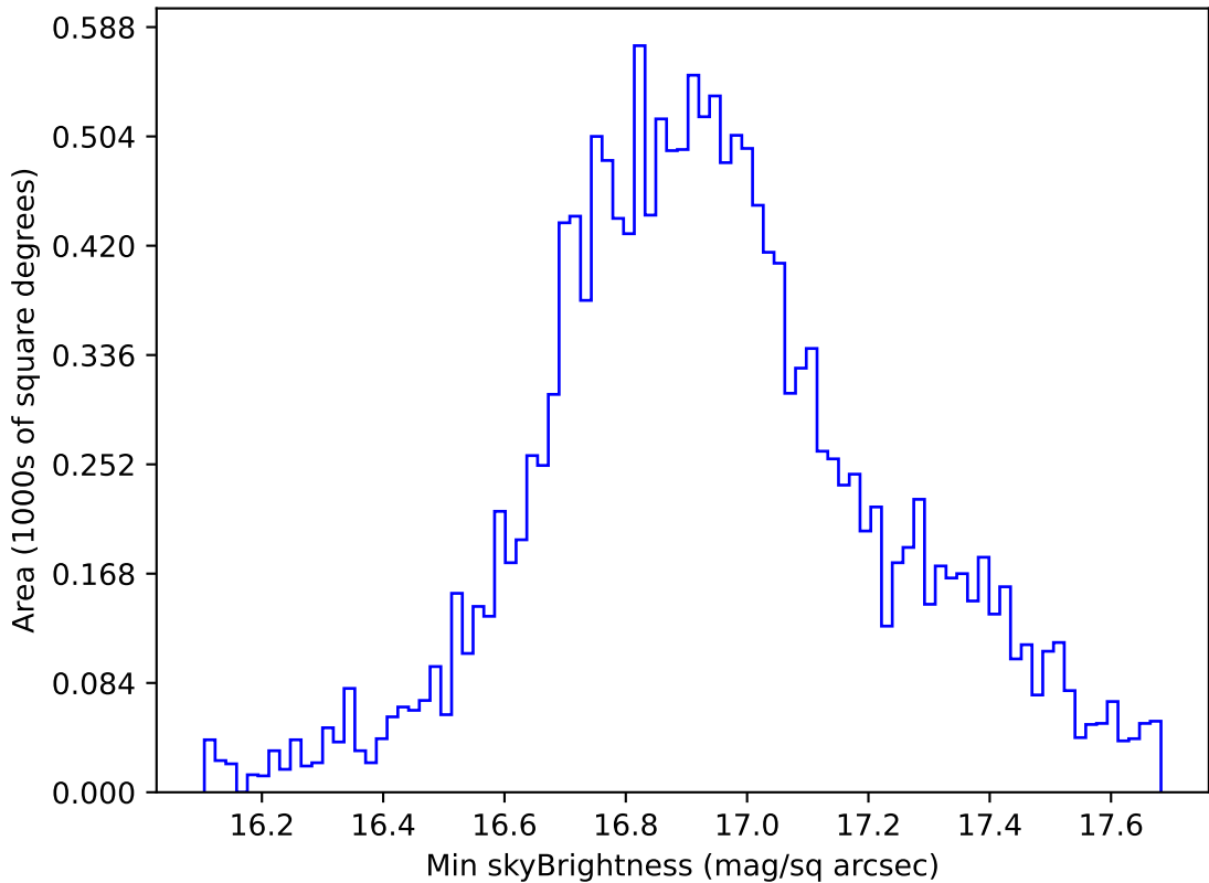
ddf_loaded_half_fl15_v3.4_10yrs WFD all bands: Min skyBrightness
