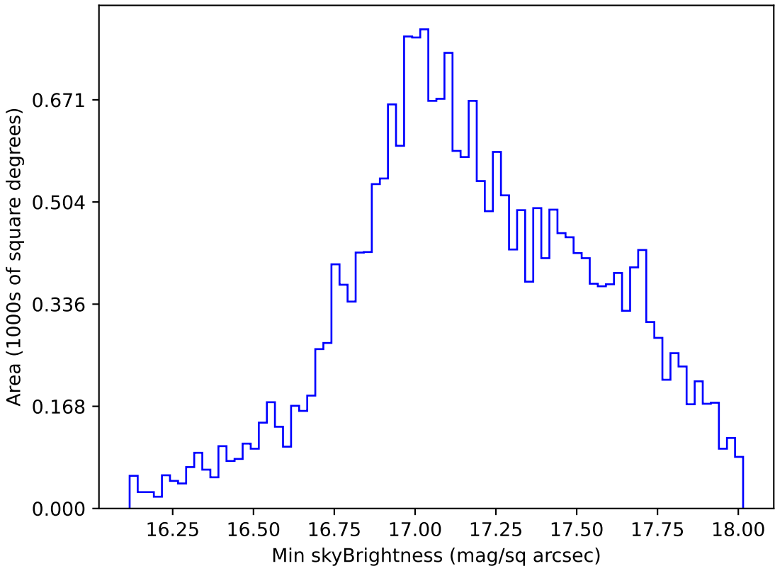
ddf_loaded_half_fl15_v3.4_10yrs All sky y band: Min skyBrightness
