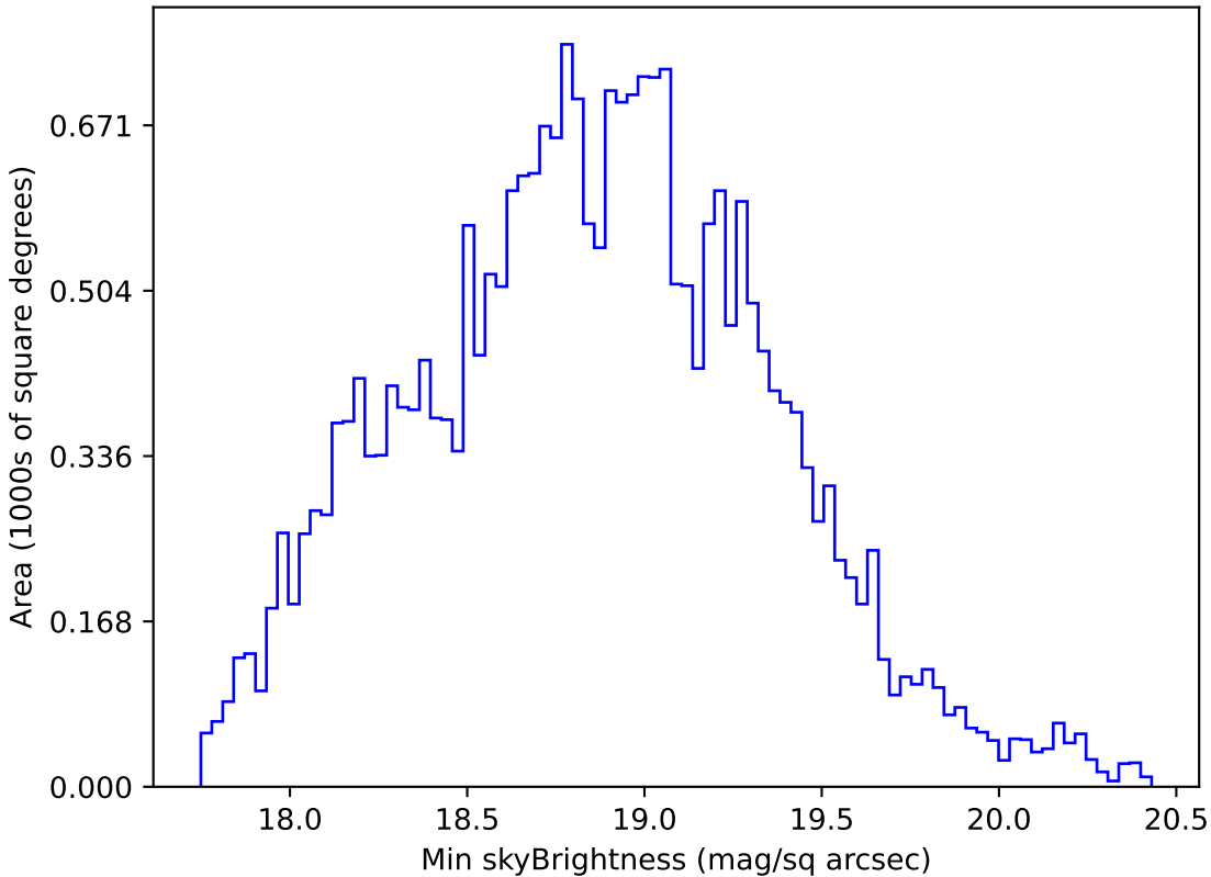
ddf_loaded_half_fl15_v3.4_10yrs All sky r band: Min skyBrightness
