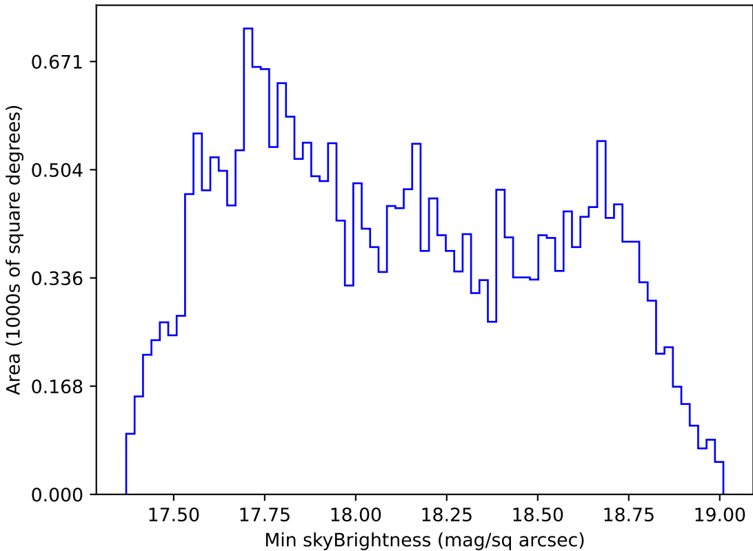
ddf_loaded_half_fl15_v3.4_10yrs All sky i band: Min skyBrightness
