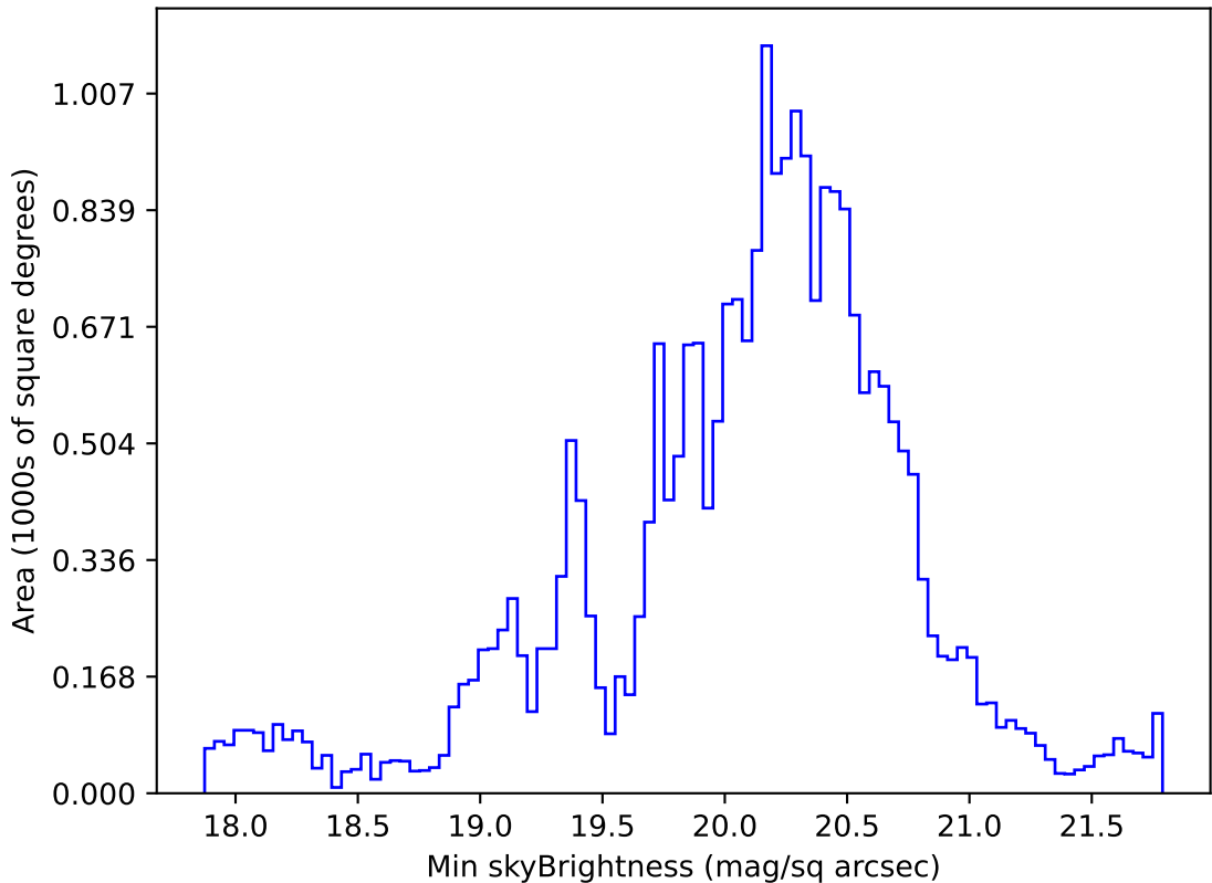
ddf_loaded_half_fl15_v3.4_10yrs All sky g band: Min skyBrightness
