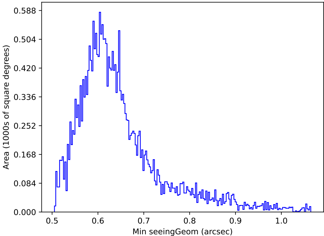
ddf_loaded_half_fl15_v3.4_10yrs Yr 1 z band: Min seeingGeom
