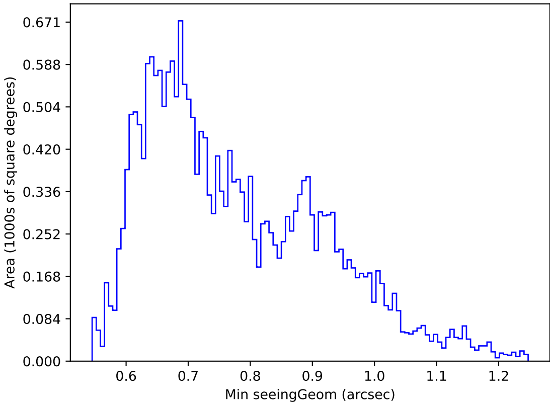
ddf_loaded_half_fl15_v3.4_10yrs Yr 1 u band: Min seeingGeom
