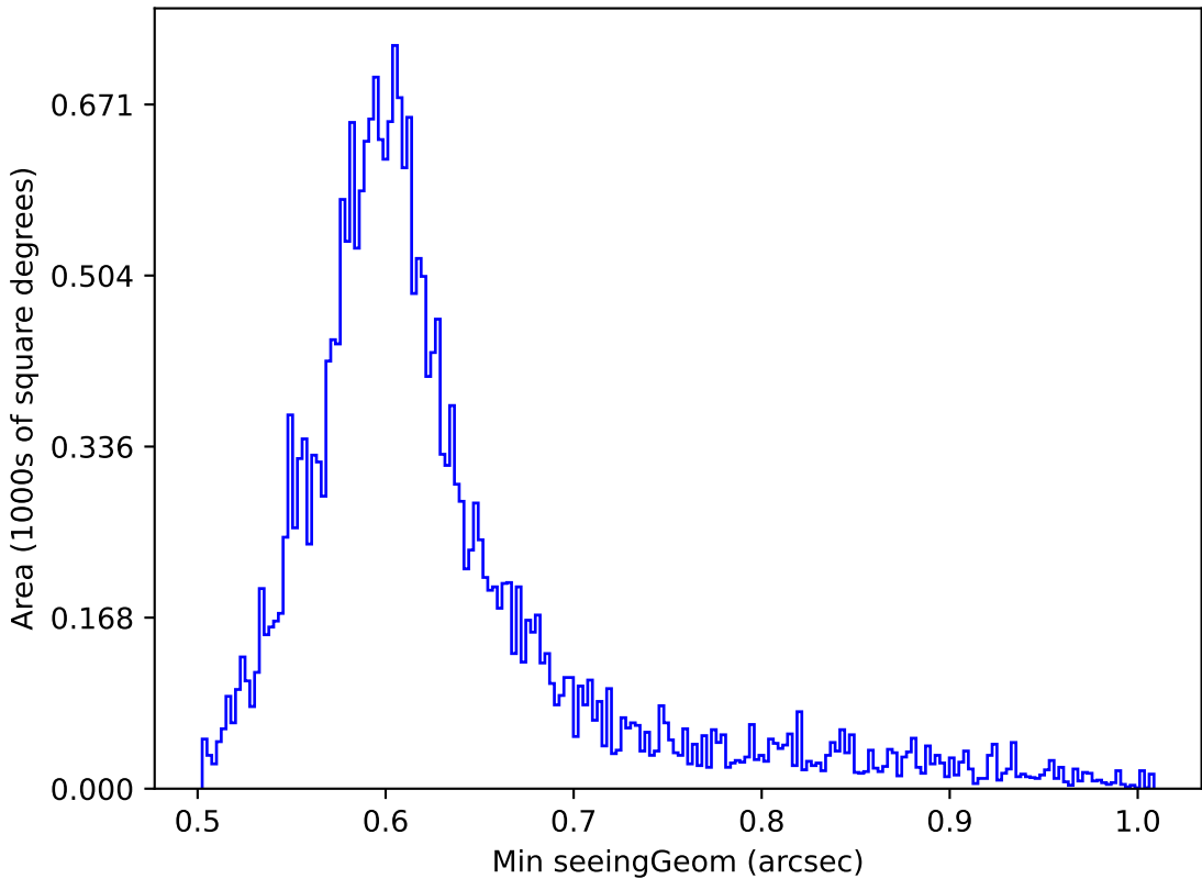
ddf_loaded_half_fl15_v3.4_10yrs Yr 1 i band: Min seeingGeom
