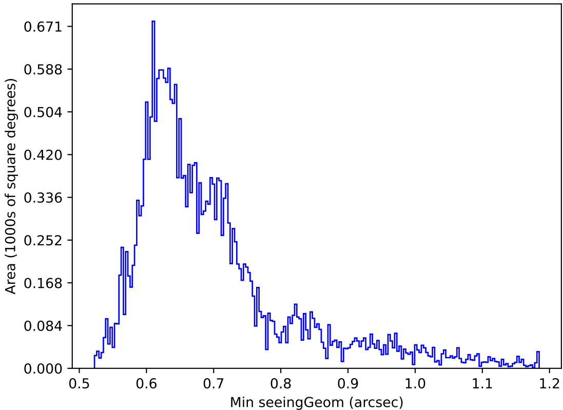
ddf_loaded_half_fl15_v3.4_10yrs Yr 1 g band: Min seeingGeom
