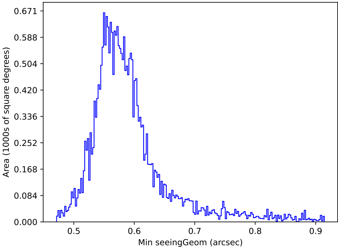
ddf_loaded_half_fl15_v3.4_10yrs Yr 1 all bands: Min seeingGeom
