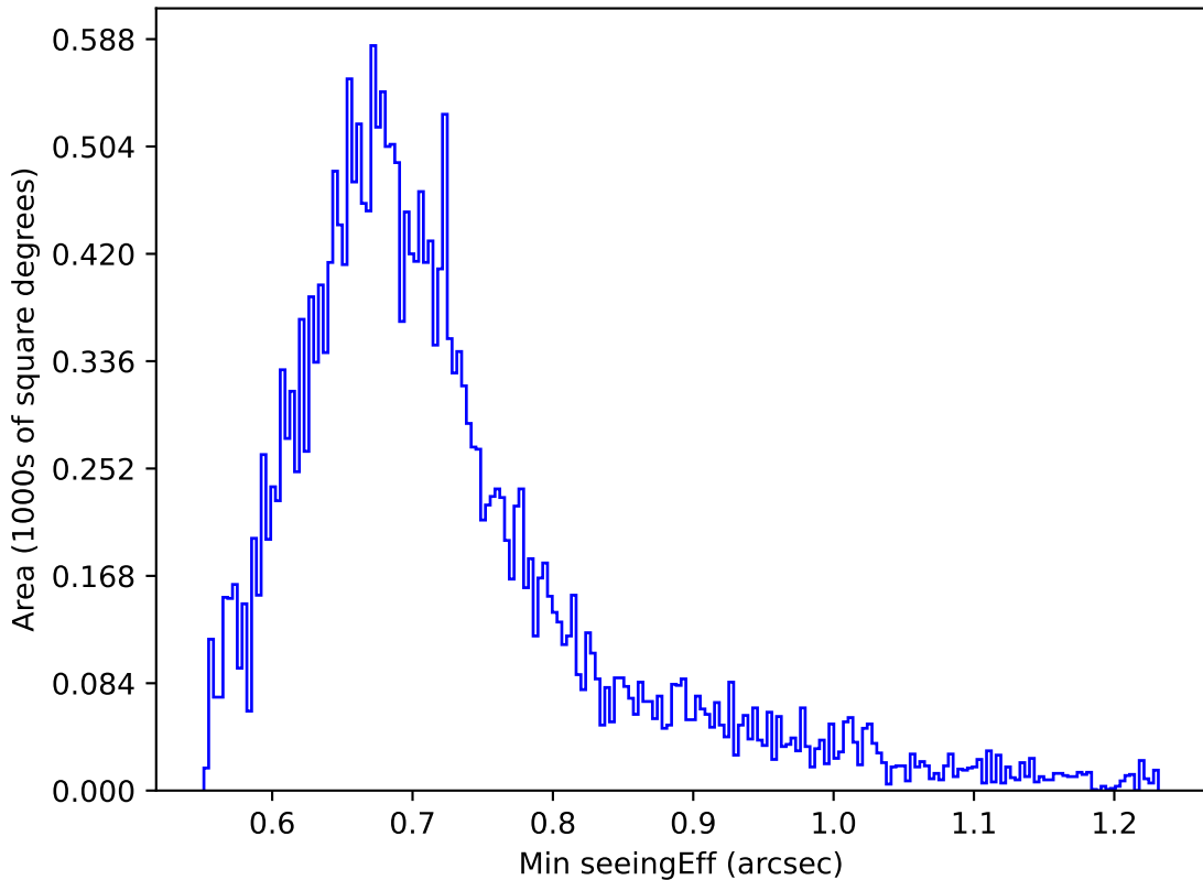
ddf_loaded_half_fl15_v3.4_10yrs Yr 1 z band: Min seeingEff
