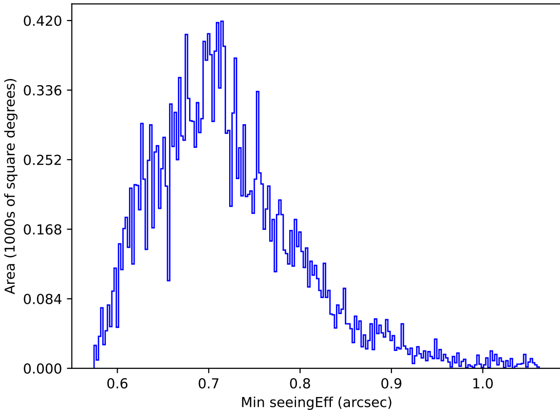
ddf_loaded_half_fl15_v3.4_10yrs Yr 1 y band: Min seeingEff
