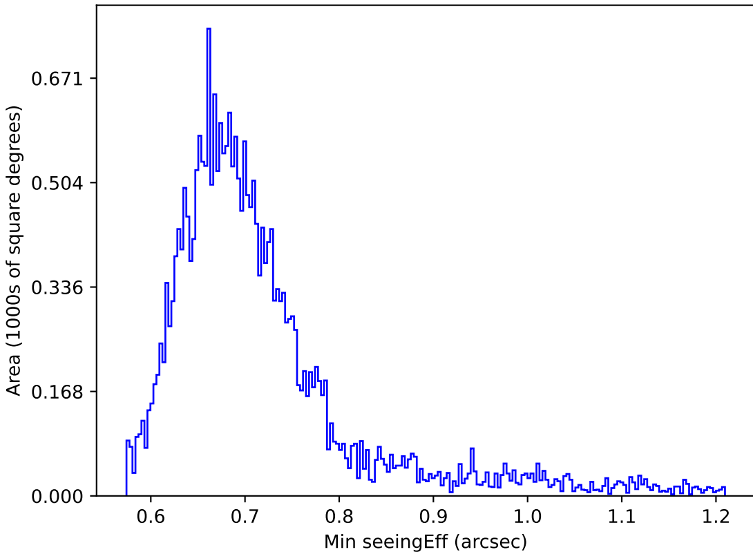
ddf_loaded_half_fl15_v3.4_10yrs Yr 1 r band: Min seeingEff
