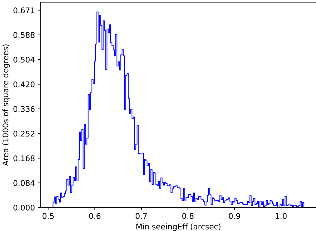
ddf_loaded_half_fl15_v3.4_10yrs Yr 1 all bands: Min seeingEff
