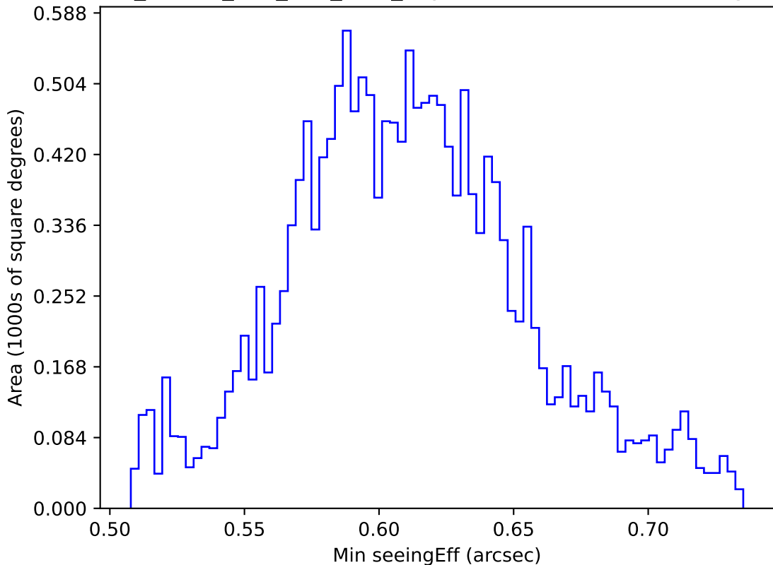
ddf_loaded_half_fl15_v3.4_10yrs WFD z band: Min seeingEff
