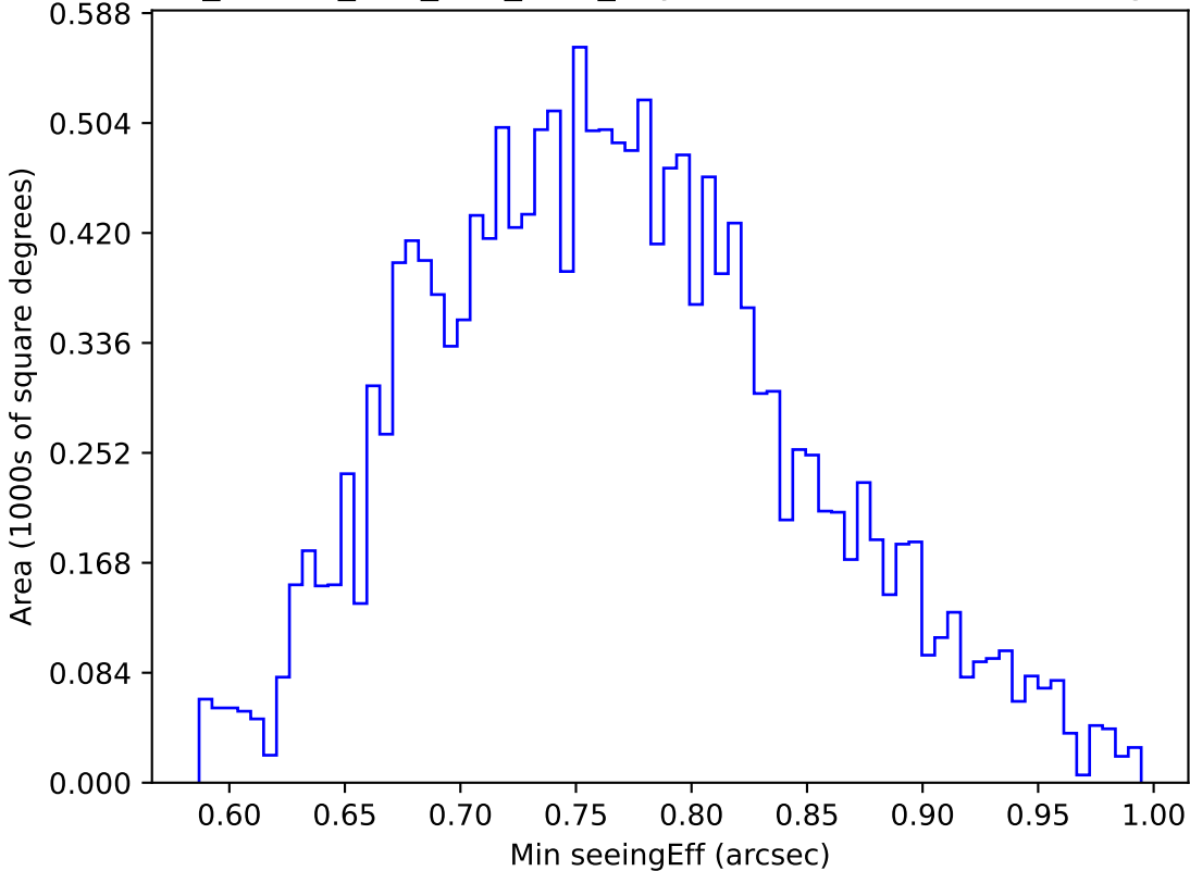
ddf_loaded_half_fl15_v3.4_10yrs WFD u band: Min seeingEff
