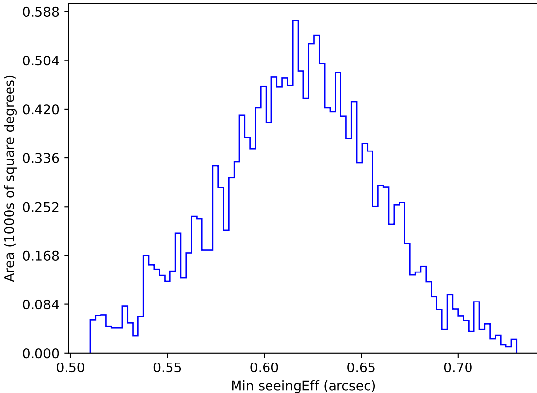
ddf_loaded_half_fl15_v3.4_10yrs WFD r band: Min seeingEff
