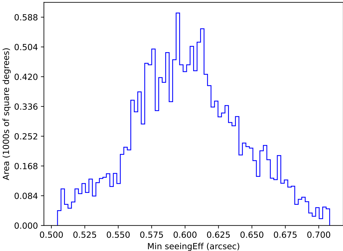
ddf_loaded_half_fl15_v3.4_10yrs WFD i band: Min seeingEff
