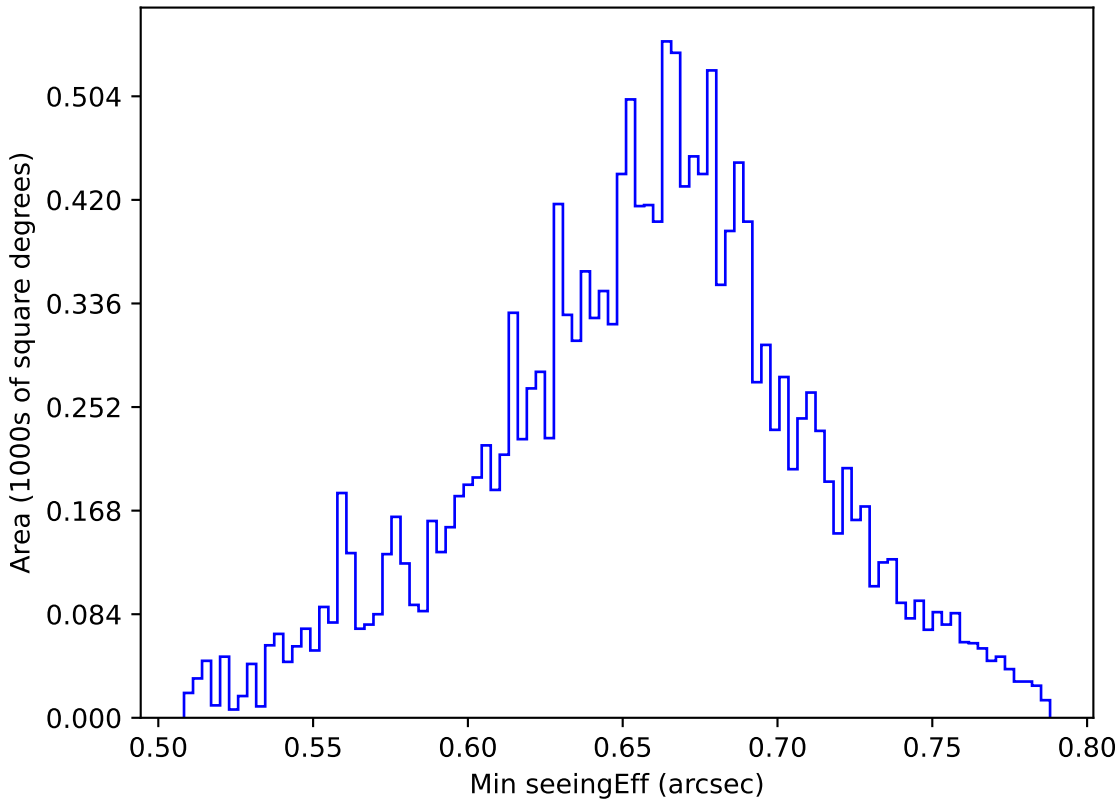
ddf_loaded_half_fl15_v3.4_10yrs WFD g band: Min seeingEff
