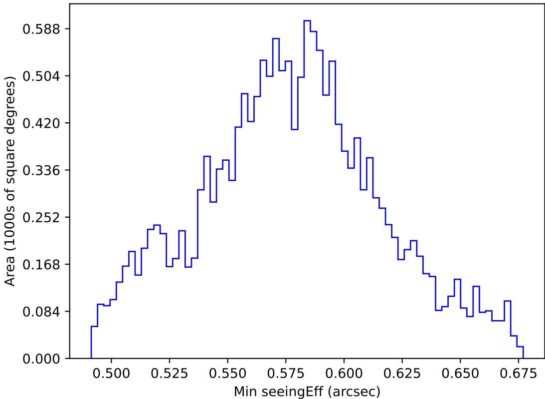
ddf_loaded_half_fl15_v3.4_10yrs WFD all bands: Min seeingEff
