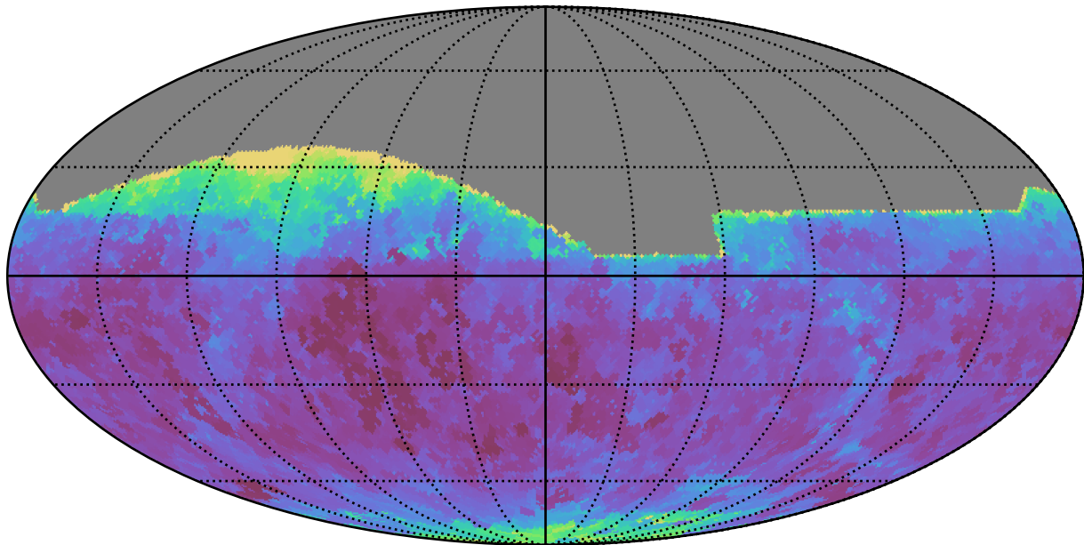
ddf_loaded_half_fl15_v3.4_10yrs All sky z band: Min seeingEff
