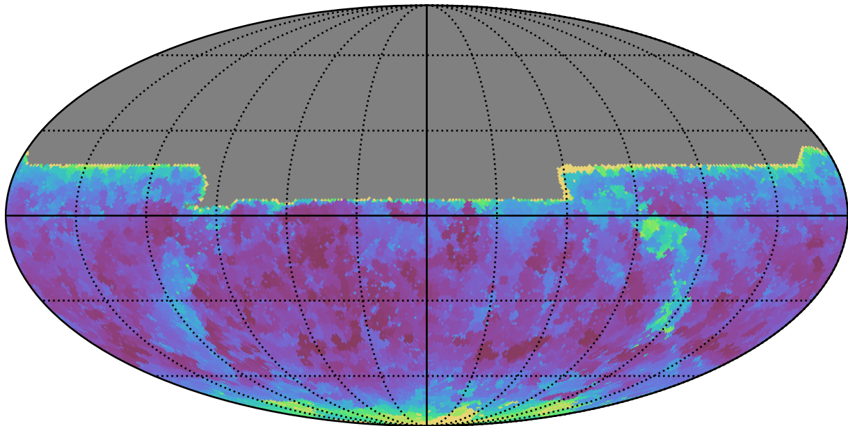
ddf_loaded_half_fl15_v3.4_10yrs All sky y band: Min seeingEff
