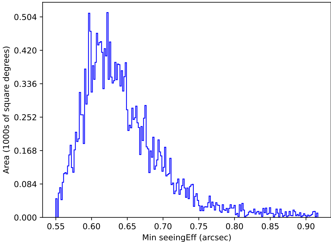
ddf_loaded_half_fl15_v3.4_10yrs All sky y band: Min seeingEff
