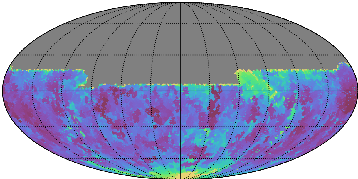
ddf_loaded_half_fl15_v3.4_10yrs All sky u band: Min seeingEff
