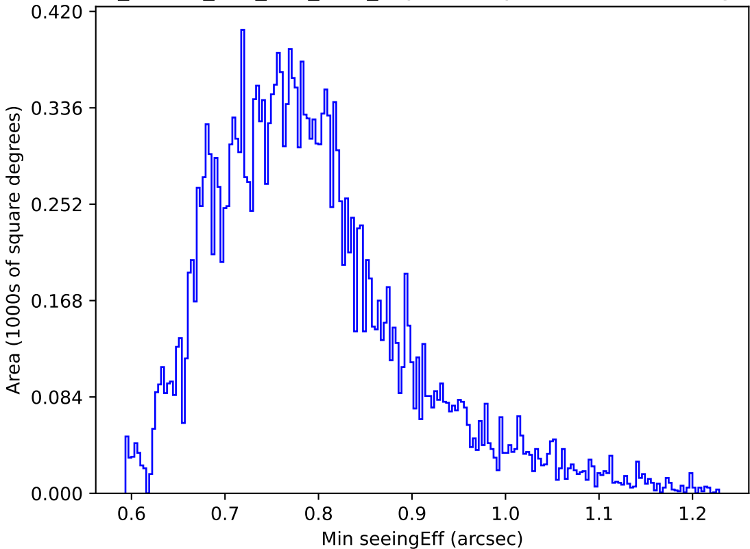
ddf_loaded_half_fl15_v3.4_10yrs All sky u band: Min seeingEff
