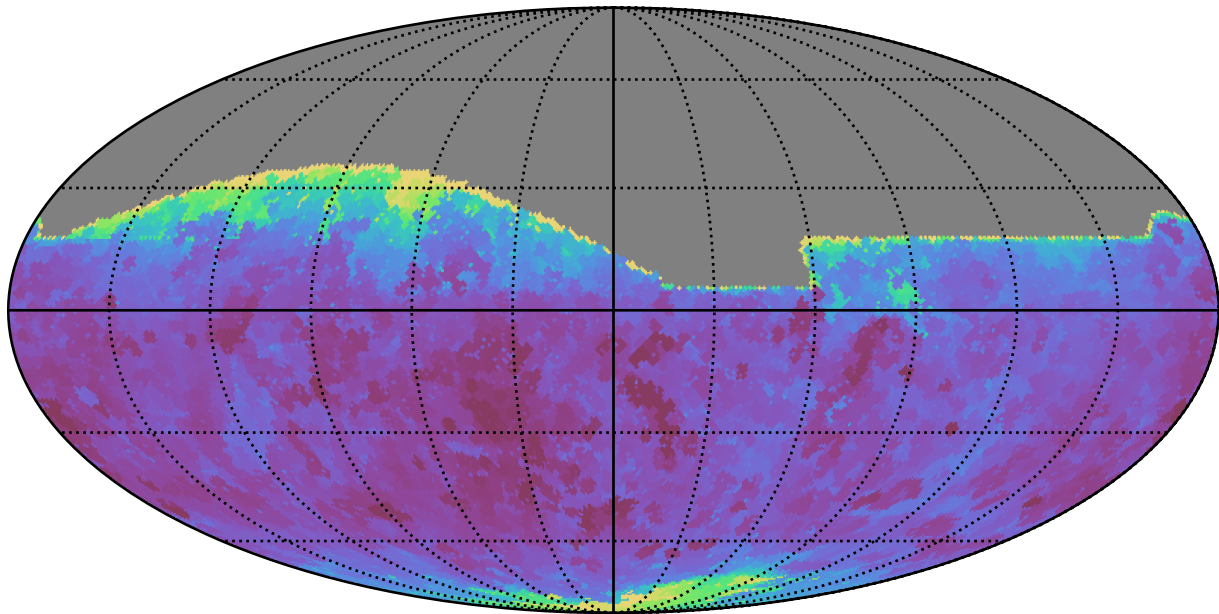
ddf_loaded_half_fl15_v3.4_10yrs All sky r band: Min seeingEff
