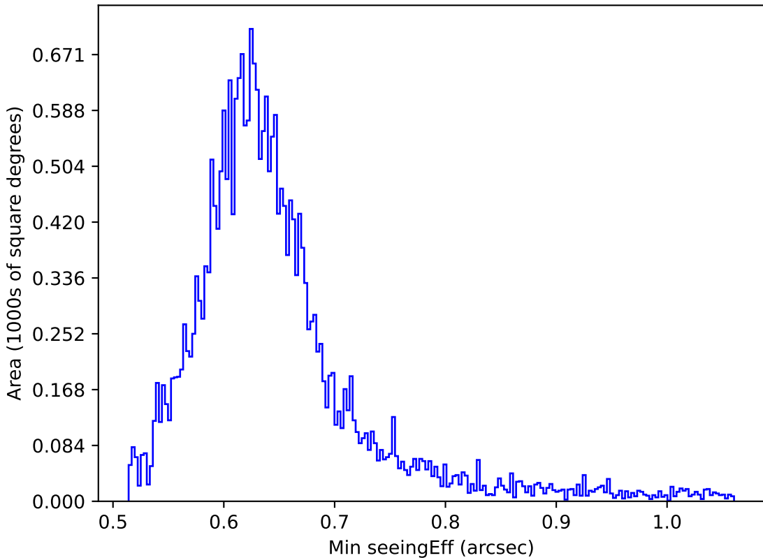
ddf_loaded_half_fl15_v3.4_10yrs All sky r band: Min seeingEff
