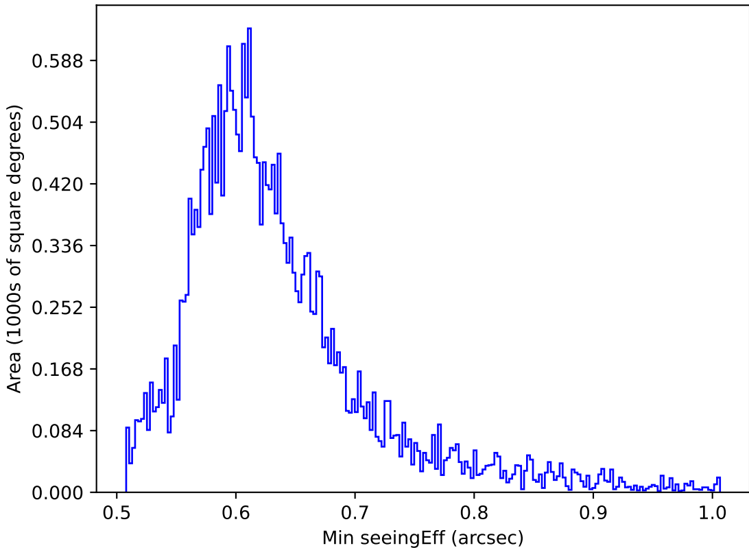
ddf_loaded_half_fl15_v3.4_10yrs All sky i band: Min seeingEff
