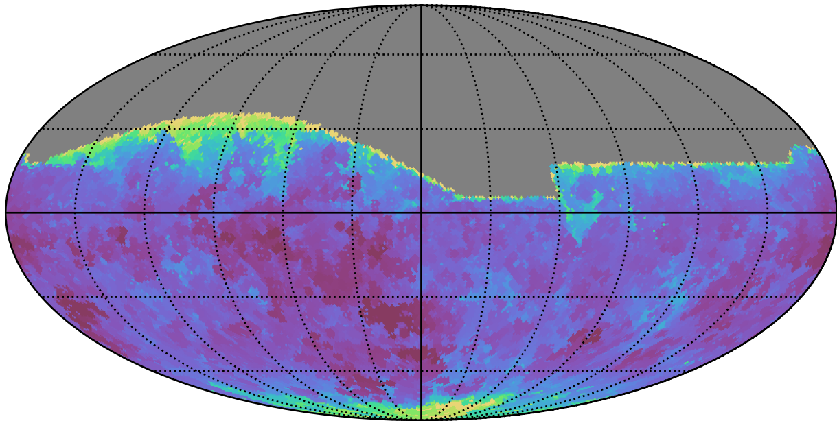
ddf_loaded_half_fl15_v3.4_10yrs All sky g band: Min seeingEff
