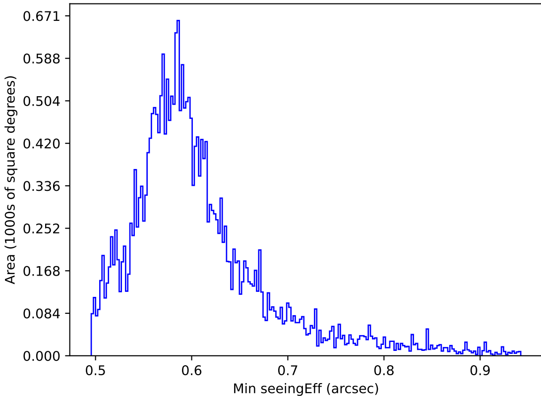
ddf_loaded_half_fl15_v3.4_10yrs All sky all bands: Min seeingEff
