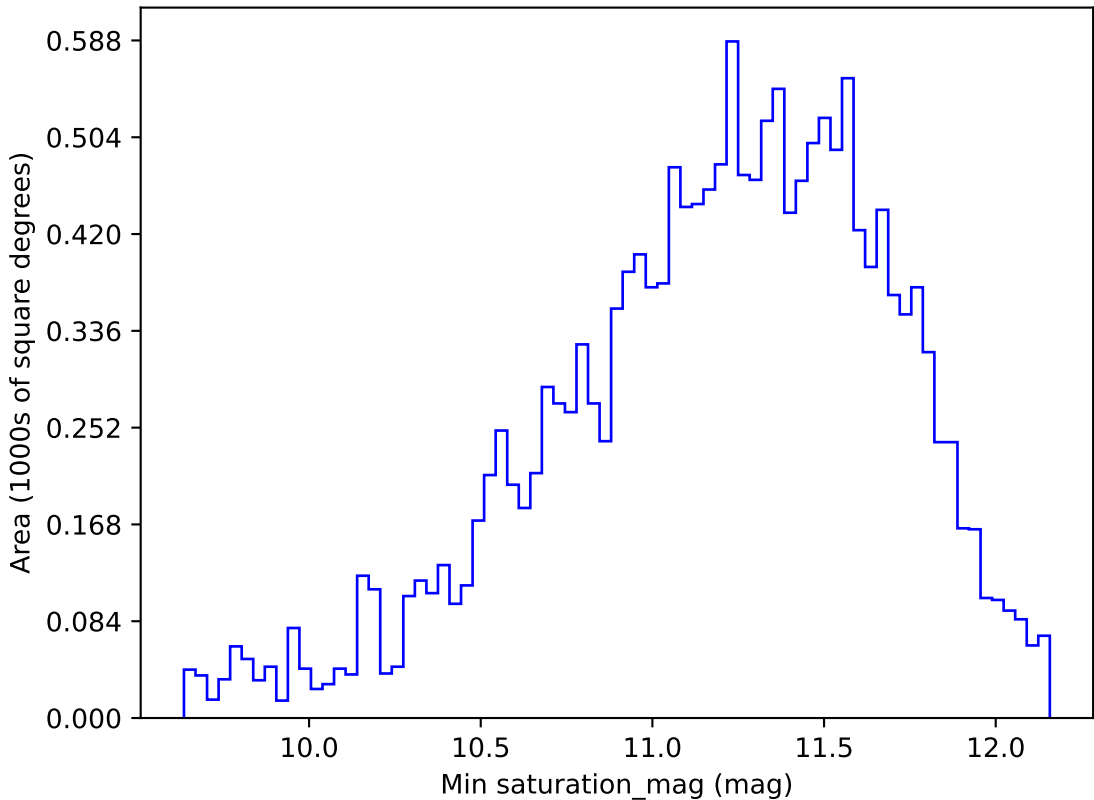
ddf_loaded_half_fl15_v3.4_10yrs WFD y band: Min saturation_mag
