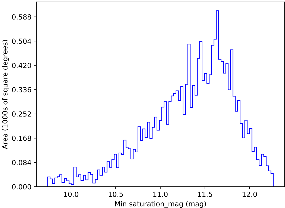
ddf_loaded_half_fl15_v3.4_10yrs WFD u band: Min saturation_mag
