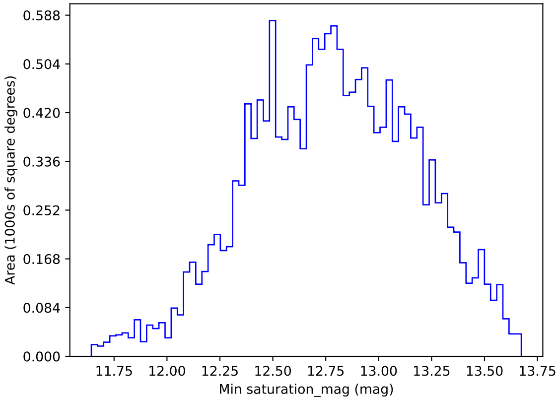
ddf_loaded_half_fl15_v3.4_10yrs WFD g band: Min saturation_mag
