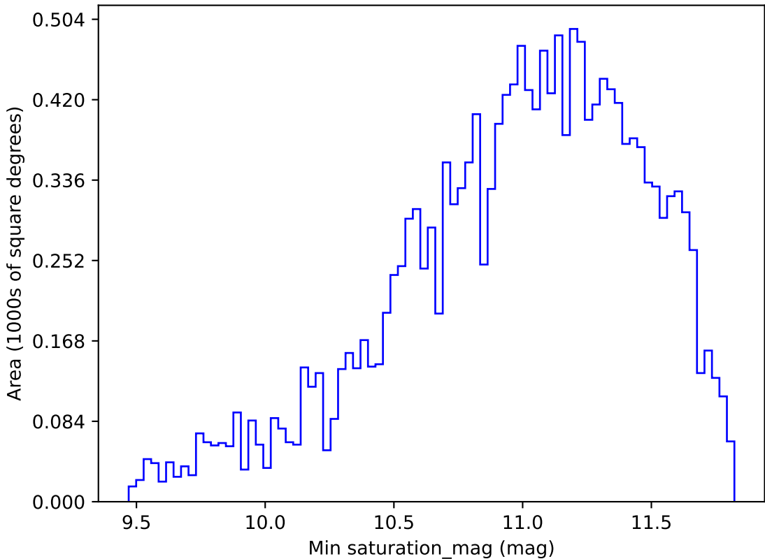
ddf_loaded_half_fl15_v3.4_10yrs WFD all bands: Min saturation_mag
