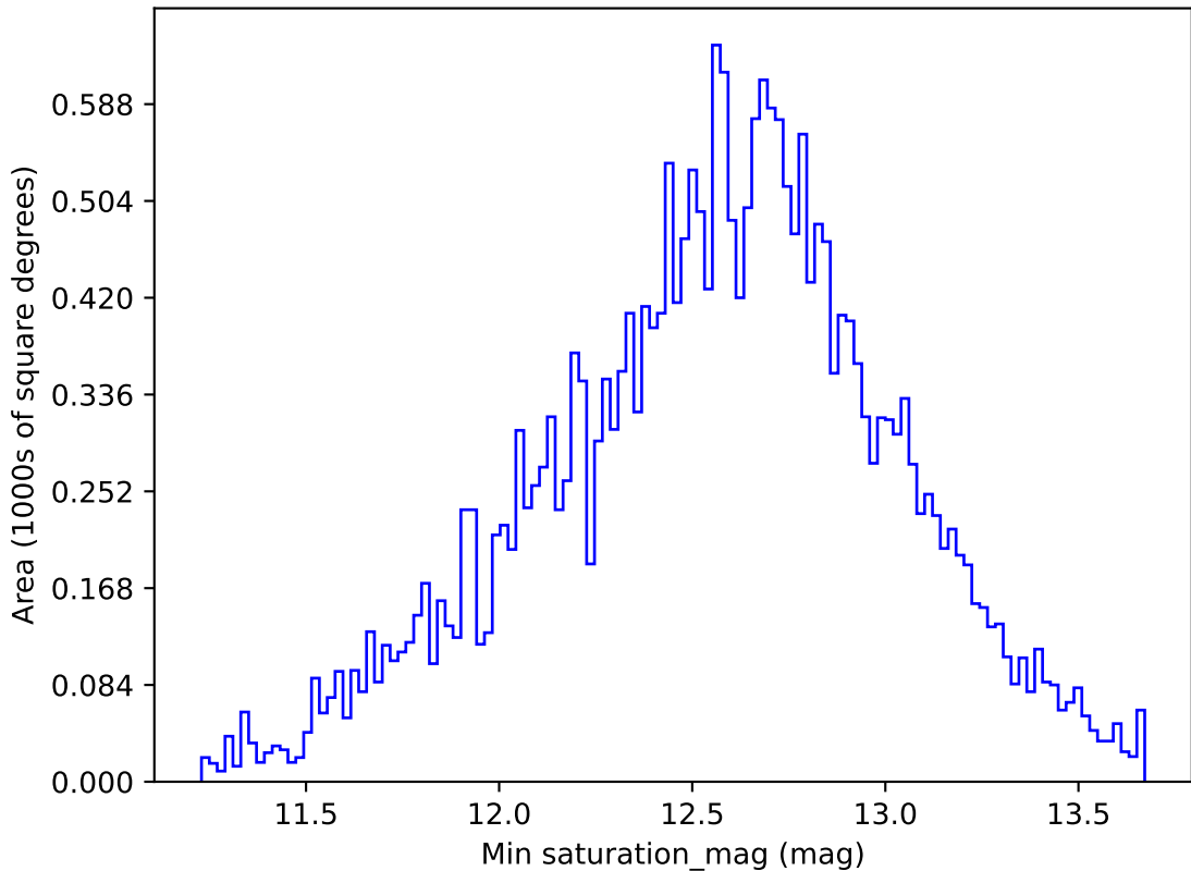
ddf_loaded_half_fl15_v3.4_10yrs All sky r band: Min saturation_mag
