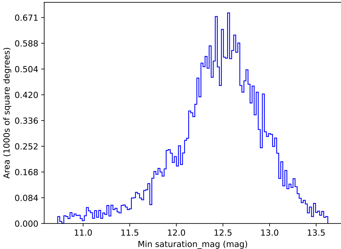
ddf_loaded_half_fl15_v3.4_10yrs All sky i band: Min saturation_mag
