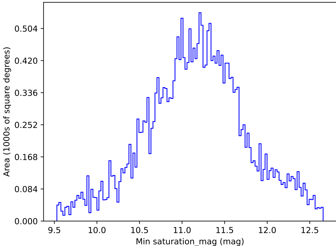
ddf_loaded_half_fl15_v3.4_10yrs All sky all bands: Min saturation_mag
