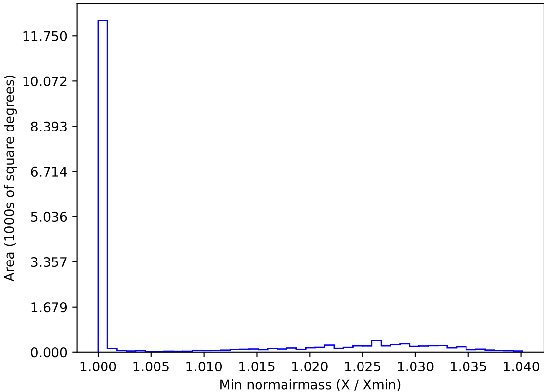
ddf_loaded_half_fl15_v3.4_10yrs WFD y band: Min normairmass
