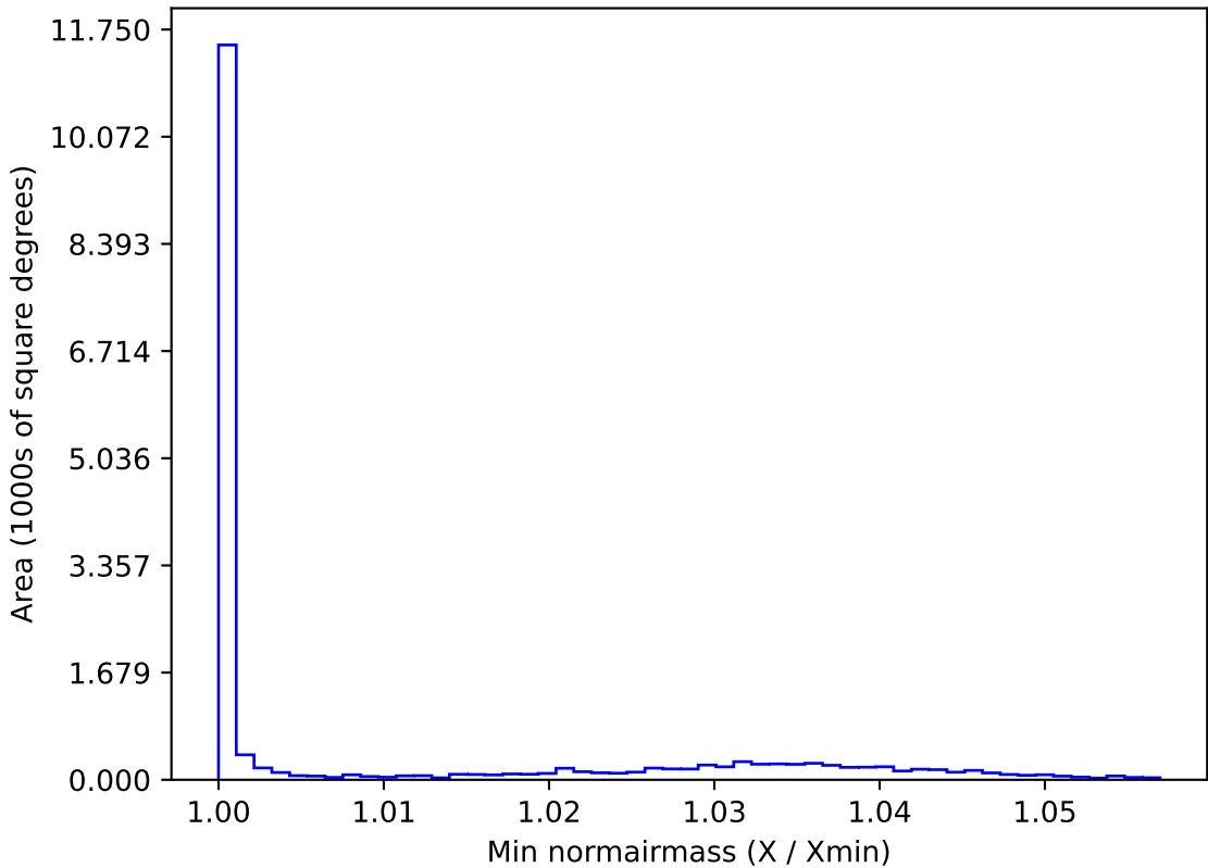
ddf_loaded_half_fl15_v3.4_10yrs WFD u band: Min normairmass
