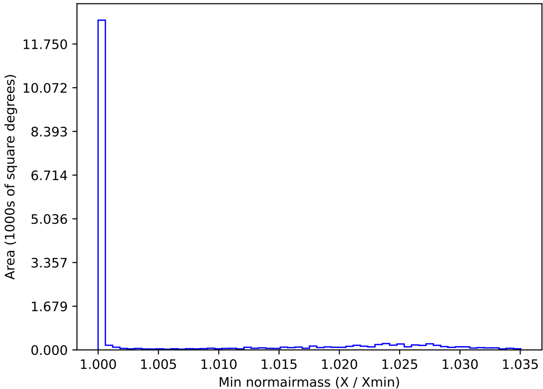
ddf_loaded_half_fl15_v3.4_10yrs WFD r band: Min normairmass
