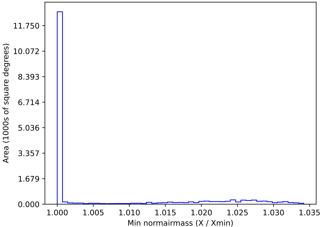
ddf_loaded_half_fl15_v3.4_10yrs WFD i band: Min normairmass
