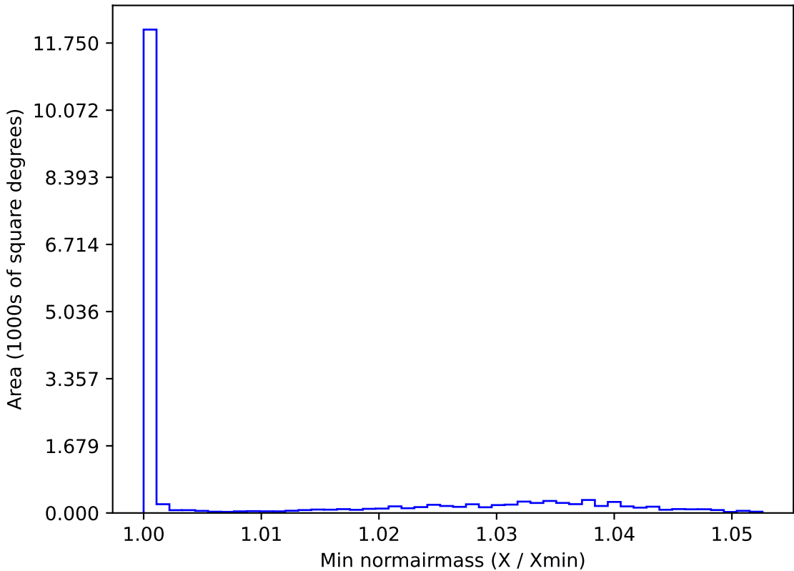
ddf_loaded_half_fl15_v3.4_10yrs WFD g band: Min normairmass
