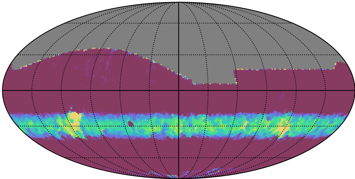
ddf_loaded_half_fl15_v3.4_10yrs All sky z band: Min normairmass
