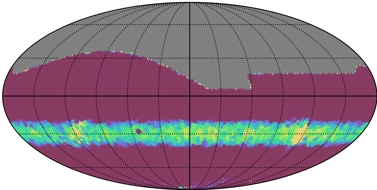
ddf_loaded_half_fl15_v3.4_10yrs All sky r band: Min normairmass
